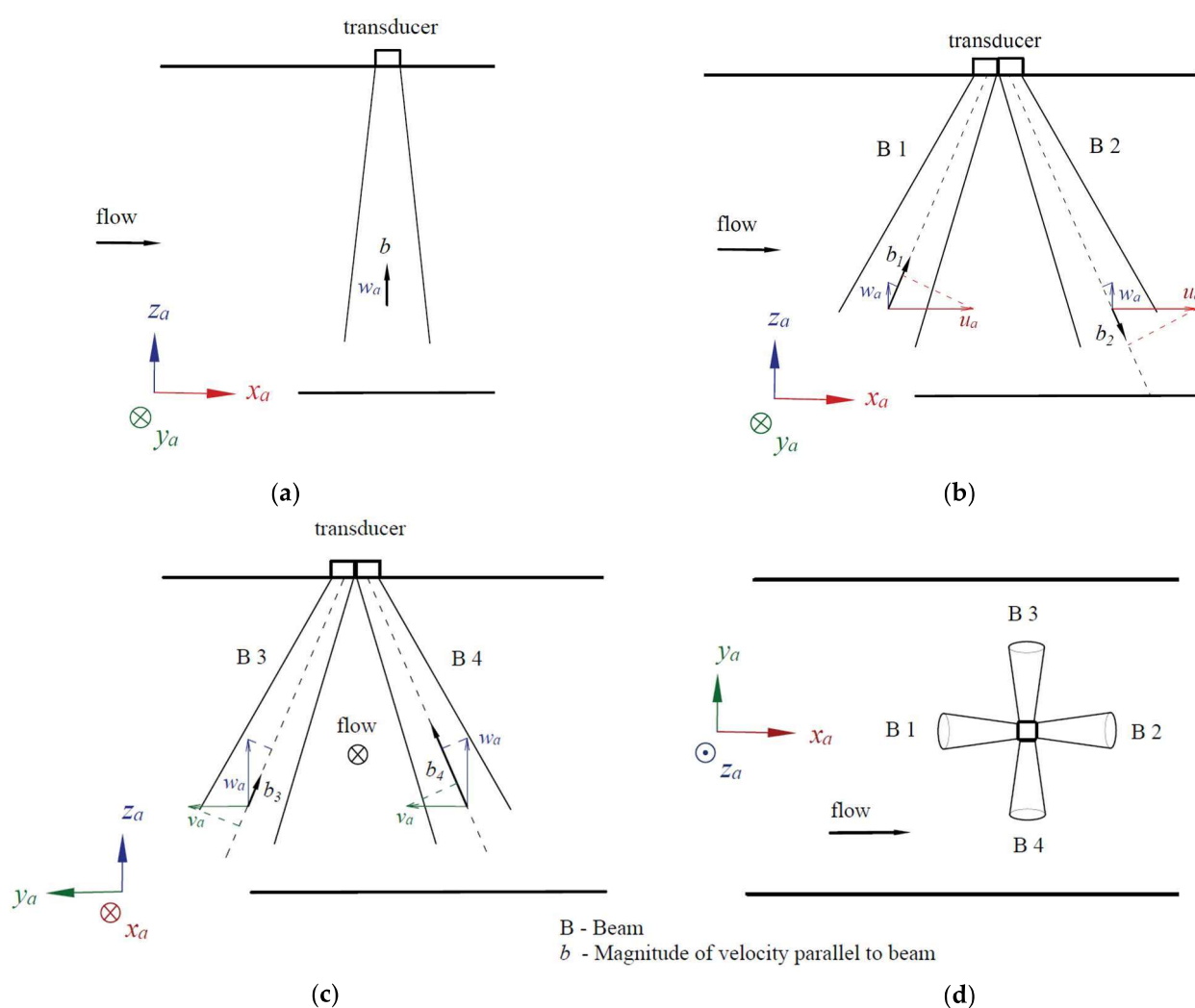
Figure 4. ADCP measured velocity and its components for (a) a single vertical beam; (b) a combination of two beams to compute stream and vertical components, u_a and w_a ; (c) a combination of beams for measuring horizontal and vertical components, v_a and w_a ; and (d) the orientation of beams from the top view to obtain the 3-dimensional current velocity in the ADCP coordinates.
