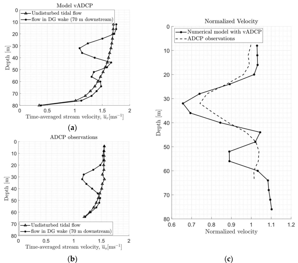
Figure 18. Time-averaged stream velocity (a) from the model vADCP and (b) the ADCP observations for undisturbed tidal flow and flow with the DG. (c) Model and observational velocity with DG, normalized with the undisturbed velocity ( \bar{u}^{DG}(z)/\bar{u}^{UG}(z) ). The velocities are measured at 70 m downstream of the Deep Green.
