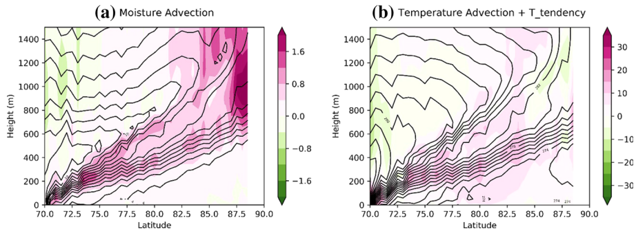
Fig. 10 Same as Fig. 9 but for a moisture advection ( \text{g kg}^{-1} \text{ day}^{-1} ), (b) temperature advection + temperature tendency due to model physics ( \text{K day}^{-1} ), along the trajectories. Black contours represent temperature (K) in (b) and specific humidity in (a)
