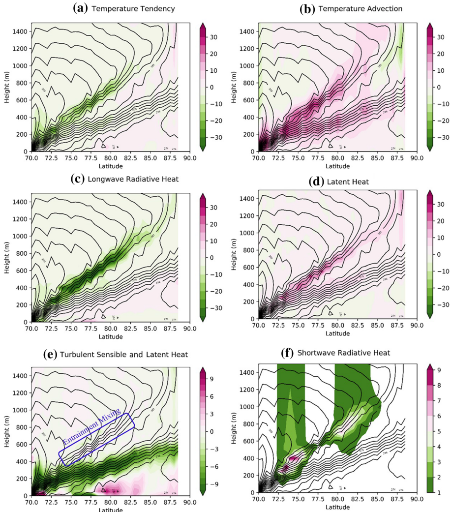
Fig. 9 Latitude–height cross-sections of ERA5 a temperature tendency due to model physics, b temperature advection, c longwave radiative heating, d latent heating, e turbulent heat, and f shortwave radiative heating along the trajectories, all in \text{K day}^{-1} . Black solid contours in all panels are the mean temperature isolines
