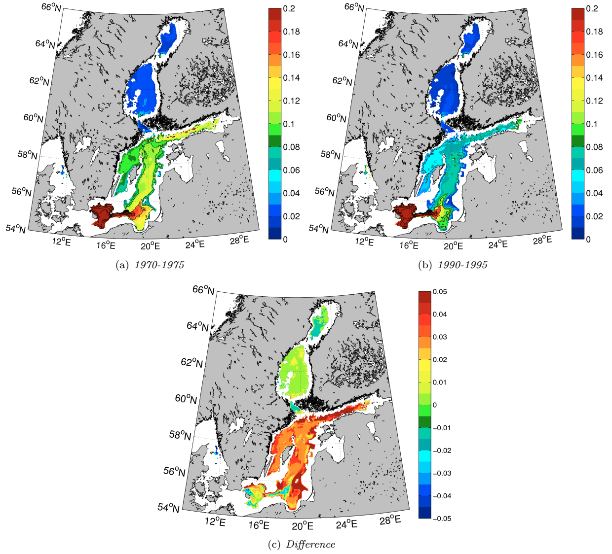
Figure 8. The mean vertical salinity gradient in the halocline for period (a) 1970-1975 and (b) 1990-1995 with (c) the difference between the periods. Units g/kg m -1 .
