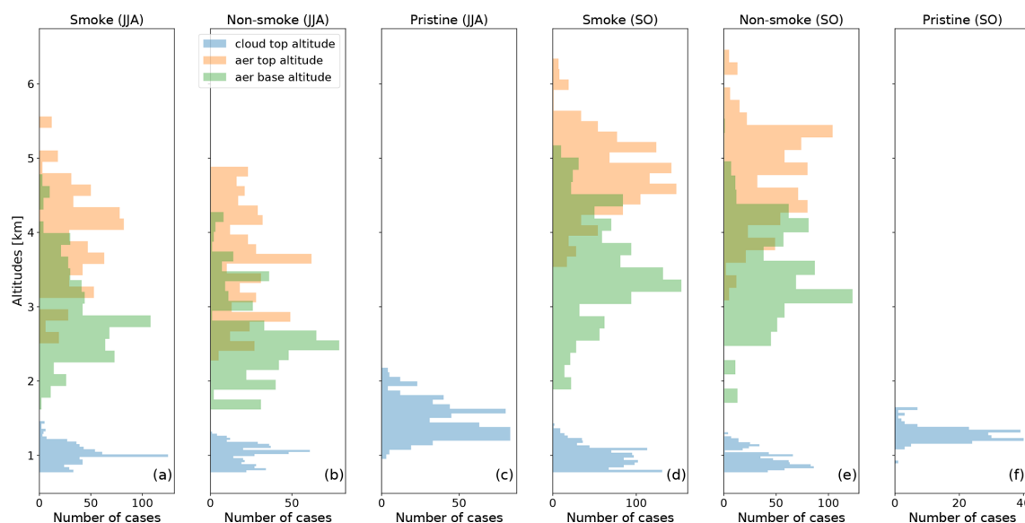
Figure 3. Altitudes of the cloud top and the aerosol (aer) top and base layers found within the area of study (latitudes from 10 to 18° S and longitudes from 2 to 10° E) during June–July–August (JJA) and September–October (SO) in the period 2007–2010. Aerosol cases are subdivided into smoke and non-smoke using the CALIOP V4 discrimination algorithm for the aerosol type.
