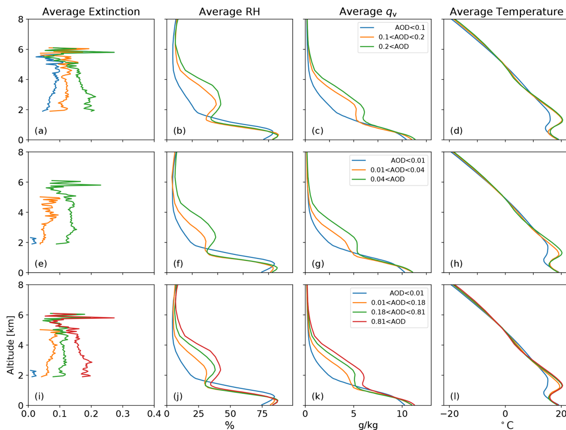
Figure A7. Mean profiles of aerosol extinction, relative humidity (RH), specific humidity ( q_v ), and temperature for CALIPSO profiles containing aerosols above clouds during the months June–July–August from 2007 to 2010. The data used for panels (a–d), (e–h), and (i–l) are exactly the same. The only difference is the selection of the interval limits and interval number for which the mean values are computed (see Sect. 3.6). The aerosol optical depth (AOD) values are obtained from the CALIPSO Aerosol Profile Data product. RH, q_v , and temperature are originally from MERRA-2 and added along the satellite track to the CALIPSO Aerosol Profile Data product.
