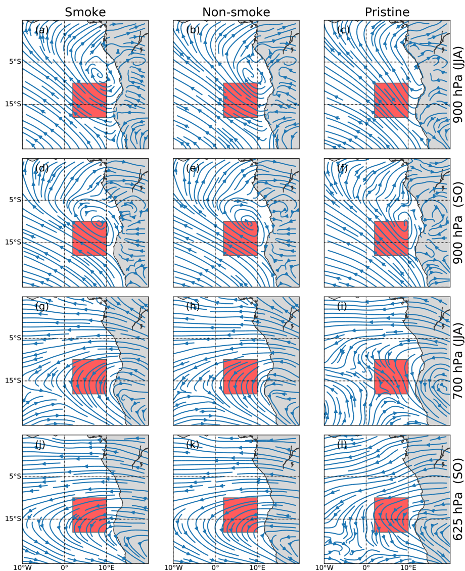
Figure 4. Streamlines corresponding to the average horizontal wind speed at 900 hPa (representative cloud level) in JJA and SO and 700 (625) hPa (representative aerosol layer level) in JJA (SO) during the days when the smoke, non-smoke aerosol, and pristine cases were identified during the period 2007–2010. The red square corresponds to the area of study.
