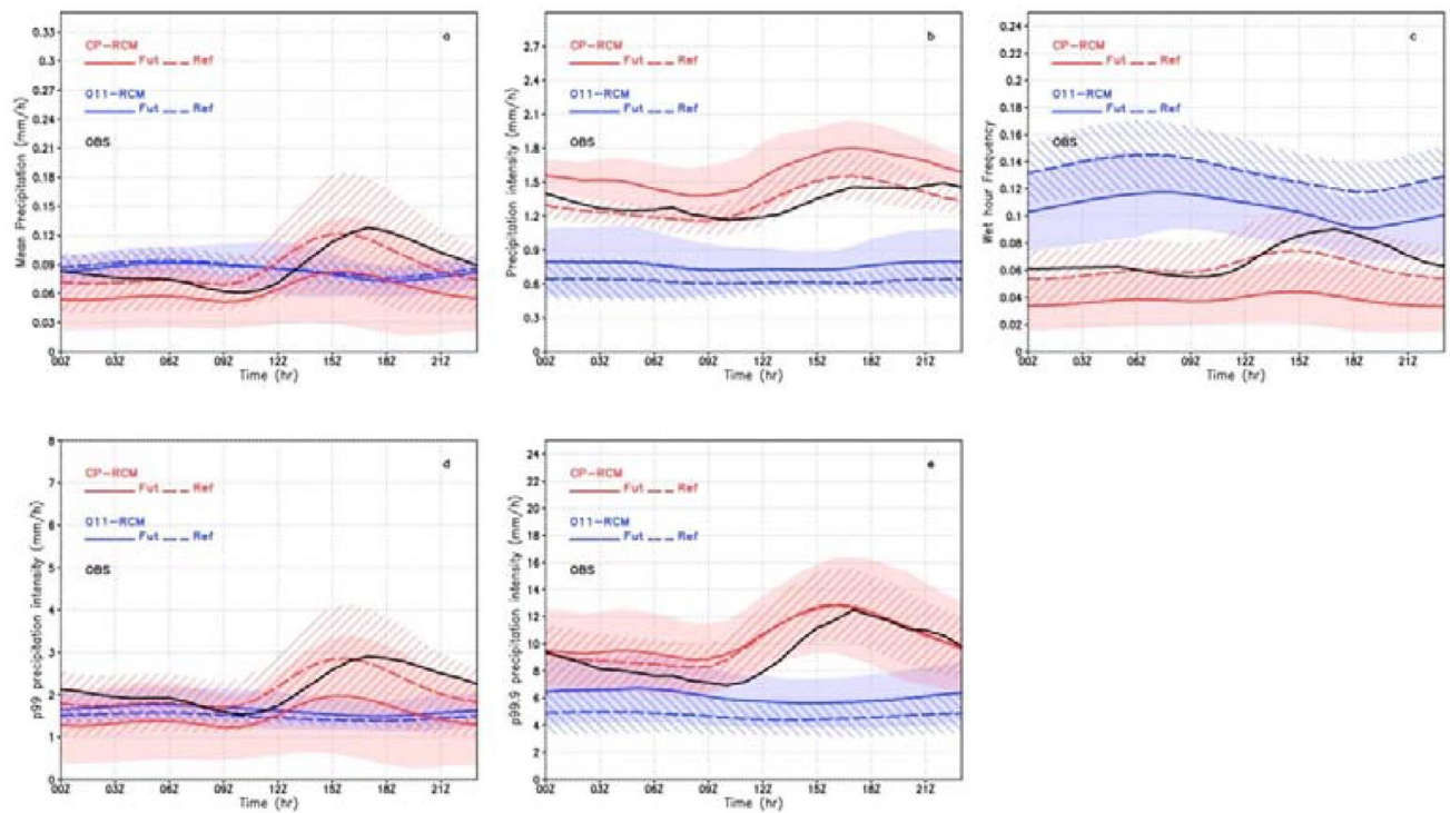
Fig. 7 As in Fig. 5 but averaged over France and with the observed COMEPHORE data (black, Sect. 3)
