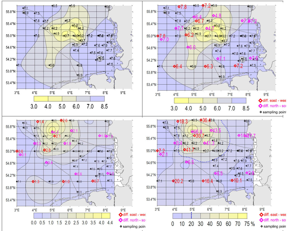
Figure 3 Method for assessing the horizontal coverage of bottom oxygen observations concentrations [top left], using the mean between adjacent observations [top right], the difference between adjacent observations [lower left] with the difference expressed as a percentage of the mean [lower right]. Only observations more than 1^{\circ} apart in longitude or 0.4^{\circ} apart in latitude, were evaluated.
