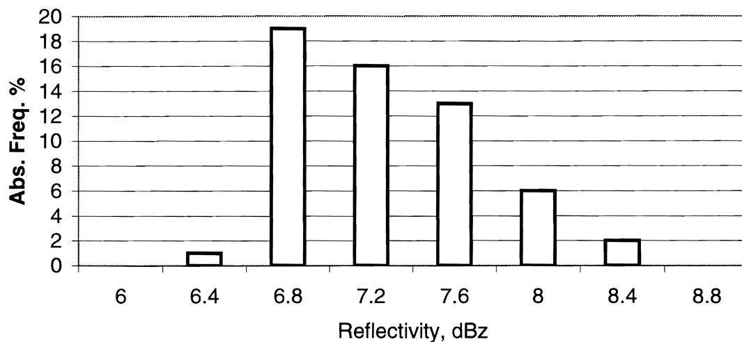
Fig. 6. The distribution is bounded to the left, since the sun signals there are below the minimum detectable signal
