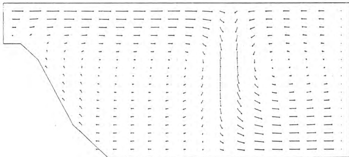
Figure 25. Small vertical diffusion ( A_v = K_v = 10 \text{ cm}^2/\text{s} )
