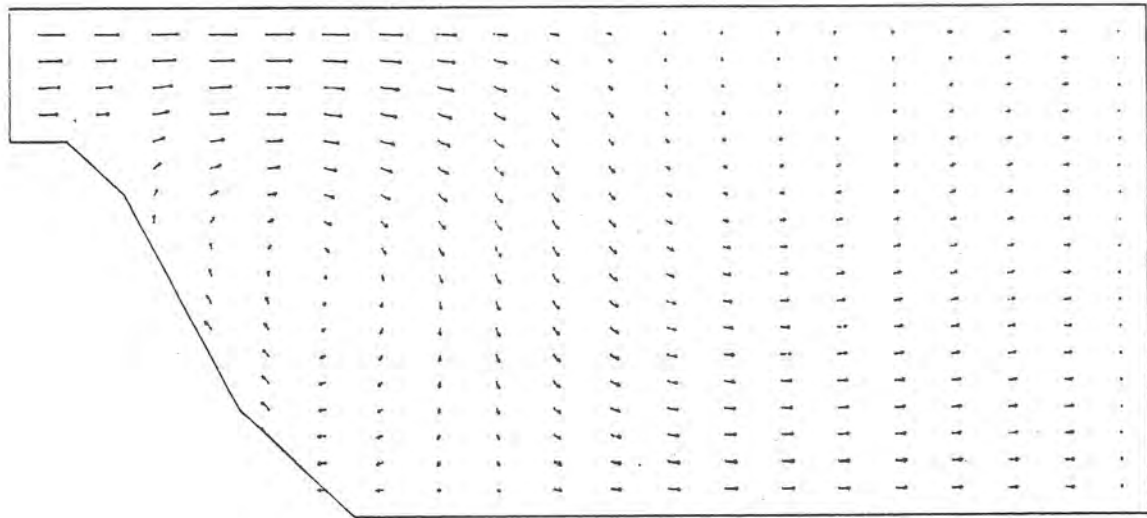
Figure 24. Big vertical diffusion ( A_v = K_v = 50 \text{ cm}^2/\text{sec} )
