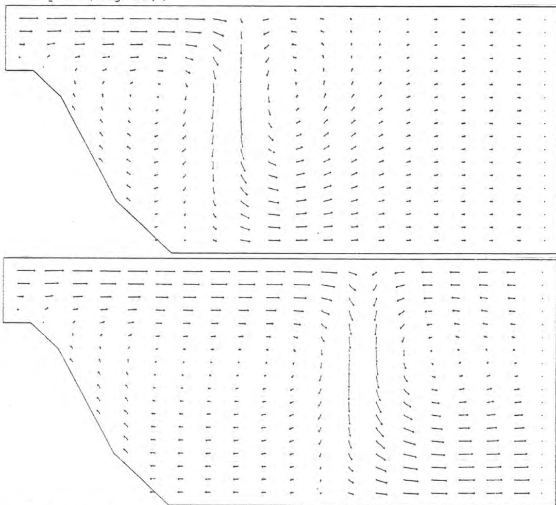
Figures 10, 11. Two stages in the development of a sinking plume (velocity vectors).
