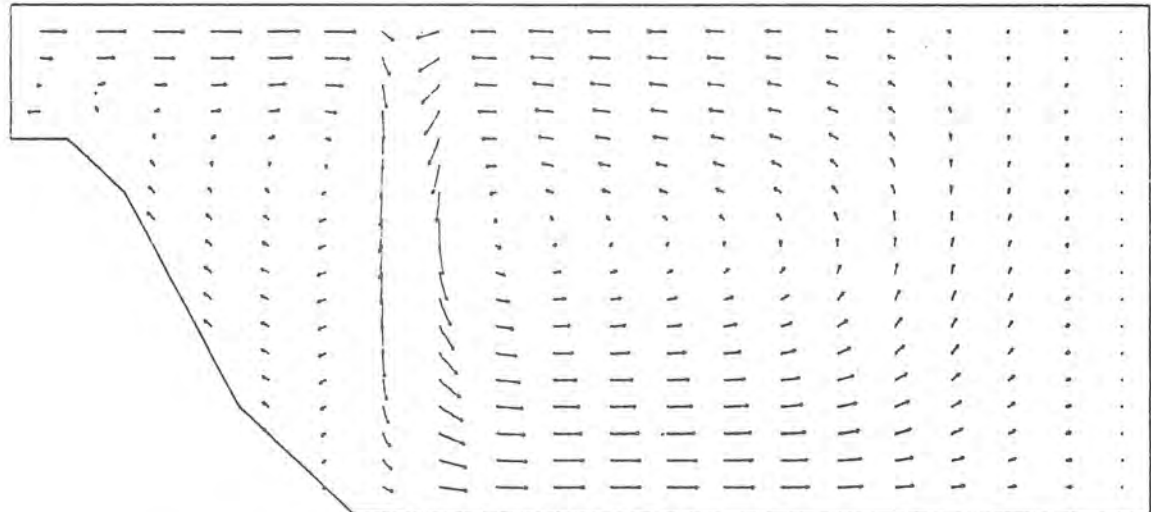
Figures 32,33. Small horizontal diffusion coefficient A_h = K_h = 2.5 \text{ m}^2/\text{sec}.
