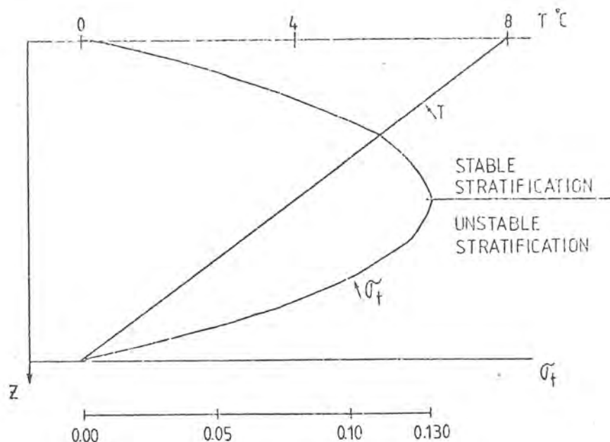
Figure 1 Density stratification for a linear temperature stratification (salinity = 0 ‰) \sigma_t = (\rho - 1) 10^3 .
