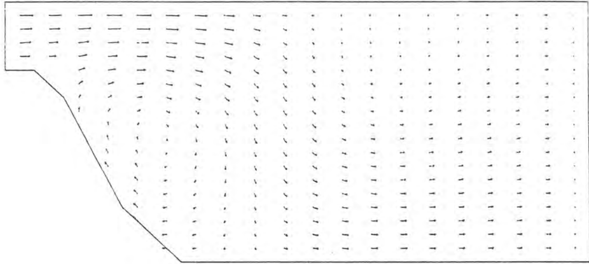
Figure 20. Plume with no heat loss to the atmosphere.
