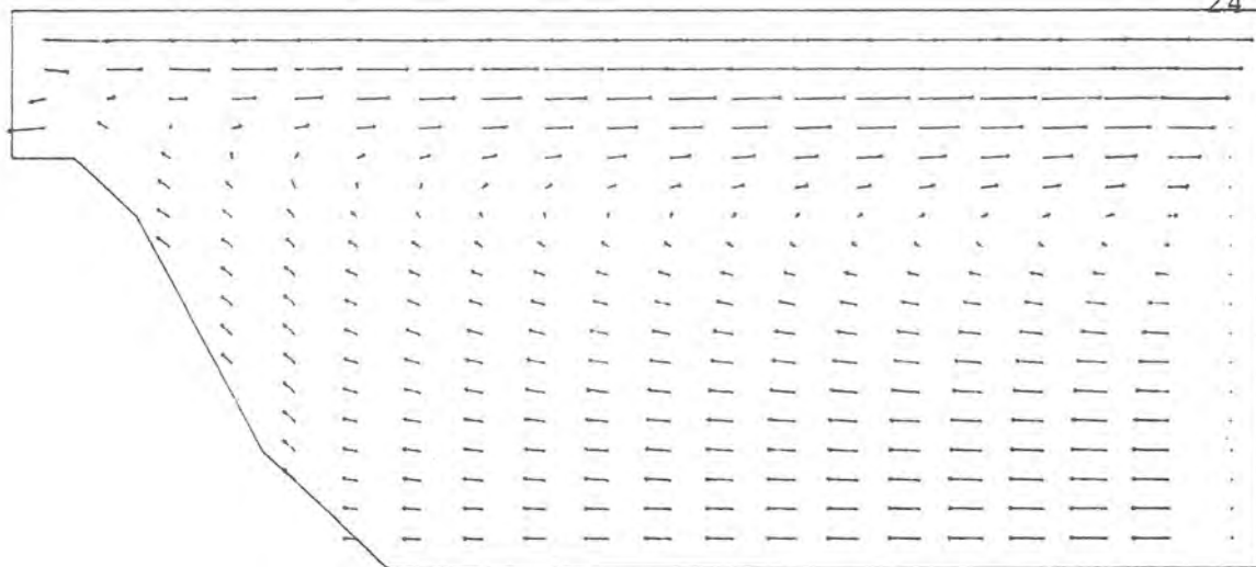
Figure 9. Floating plume, velocity vectors, horizontal scale = 20 x vertical scale.
