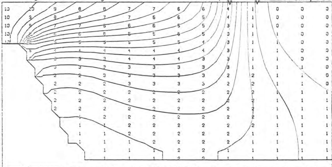
Figure 23. Small vertical diffusion ( A_v = K_v = 10 \text{ cm}^2/\text{sec} )
