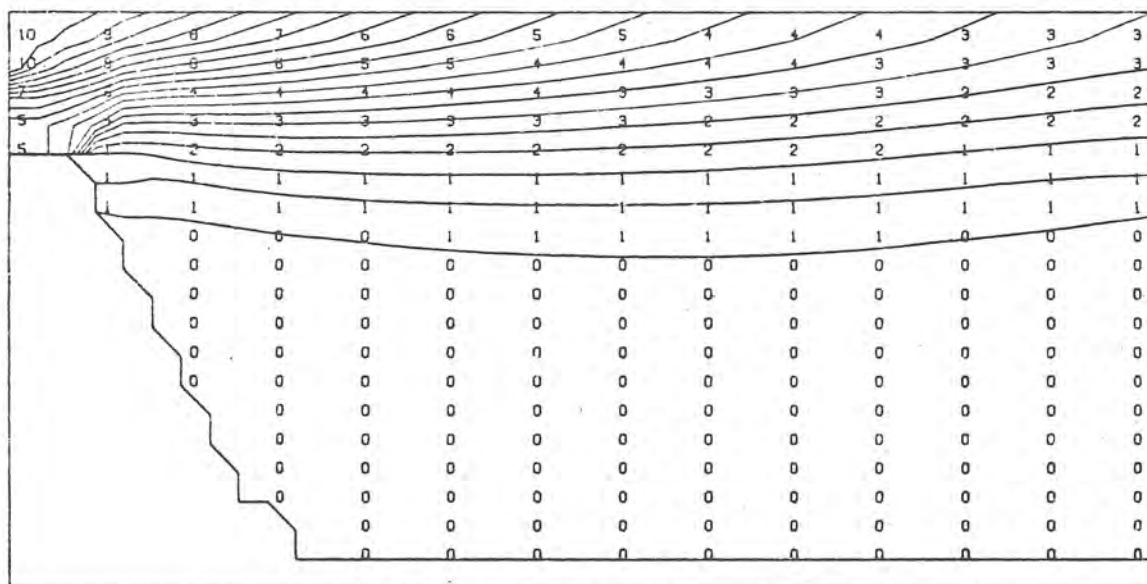
Figur 8. Floating plume ambient temperature 10^\circ\text{C} discharge temperature 20^\circ\text{C} .
