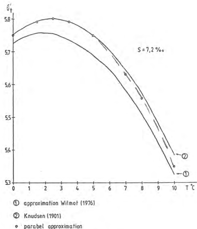
Figure 6. Different approximations for the dependence of density on temperature.
