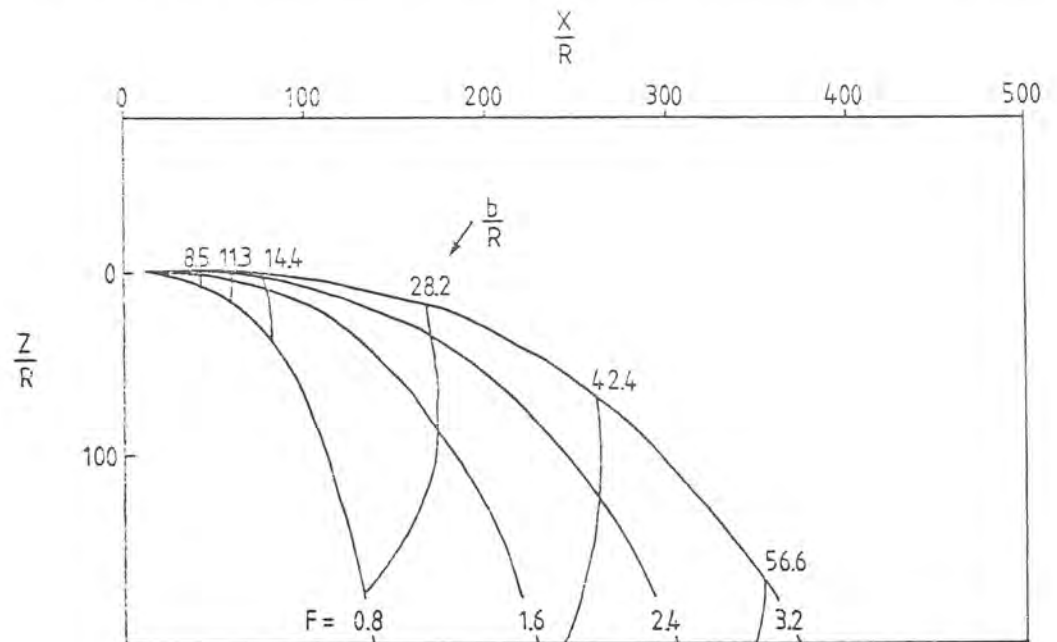
Figure 5 Centerline trajectory and half-width of round jets.
